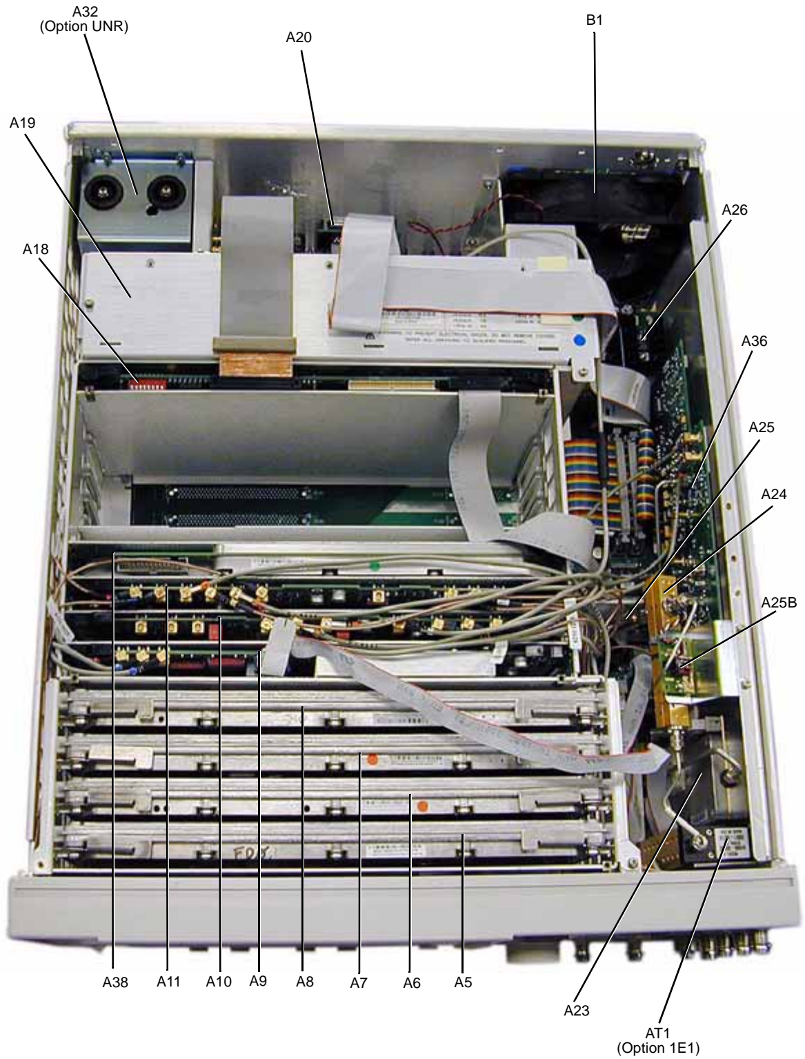
Figure 3-4 Assemblies from a Top View (E8257D Options 550 and 567)
