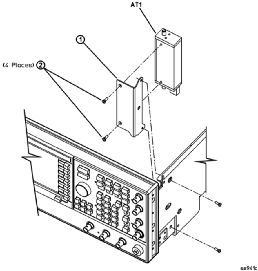
Figure 3-21 Disassembled AT1 90dB/115dB Attenuator View (Option 1E1)
