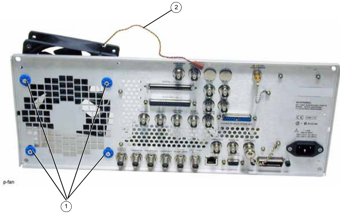
Figure 2-61 B1 Fan
