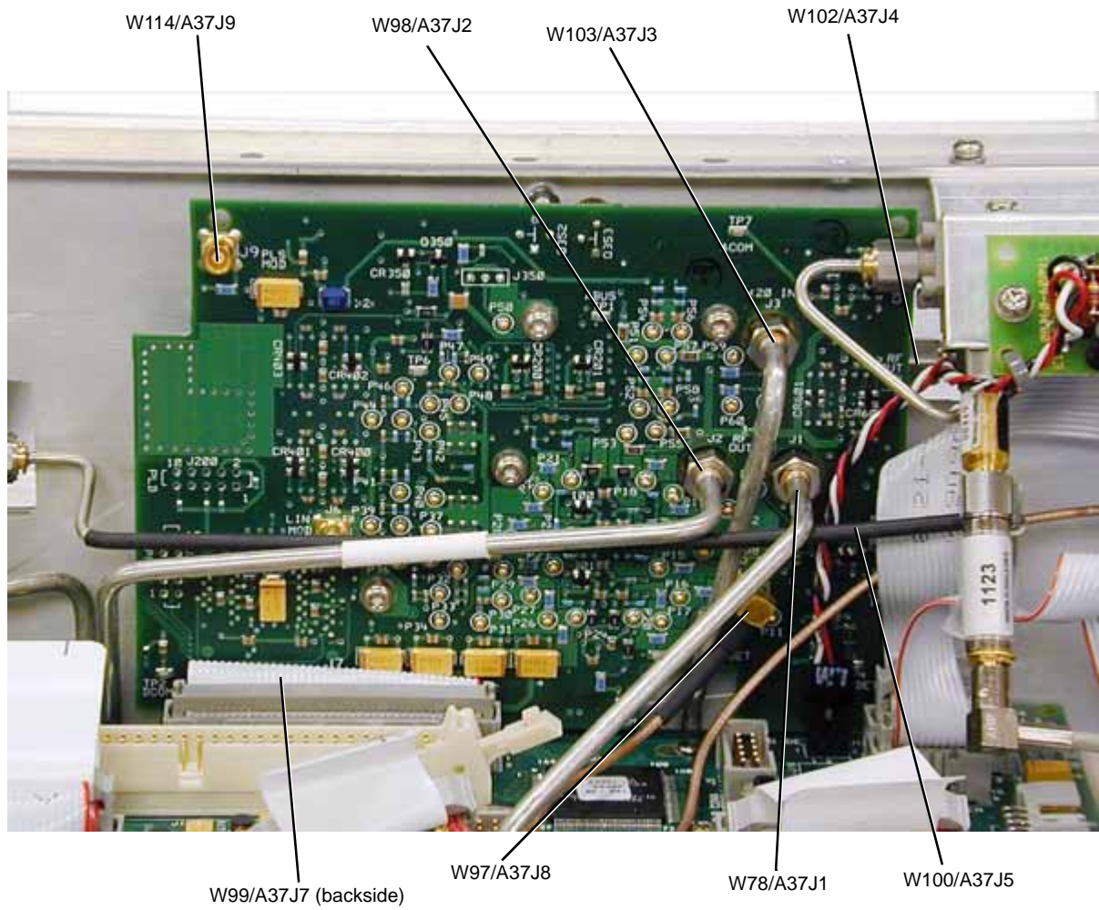
Figure 2-54 A37 Upconverter
