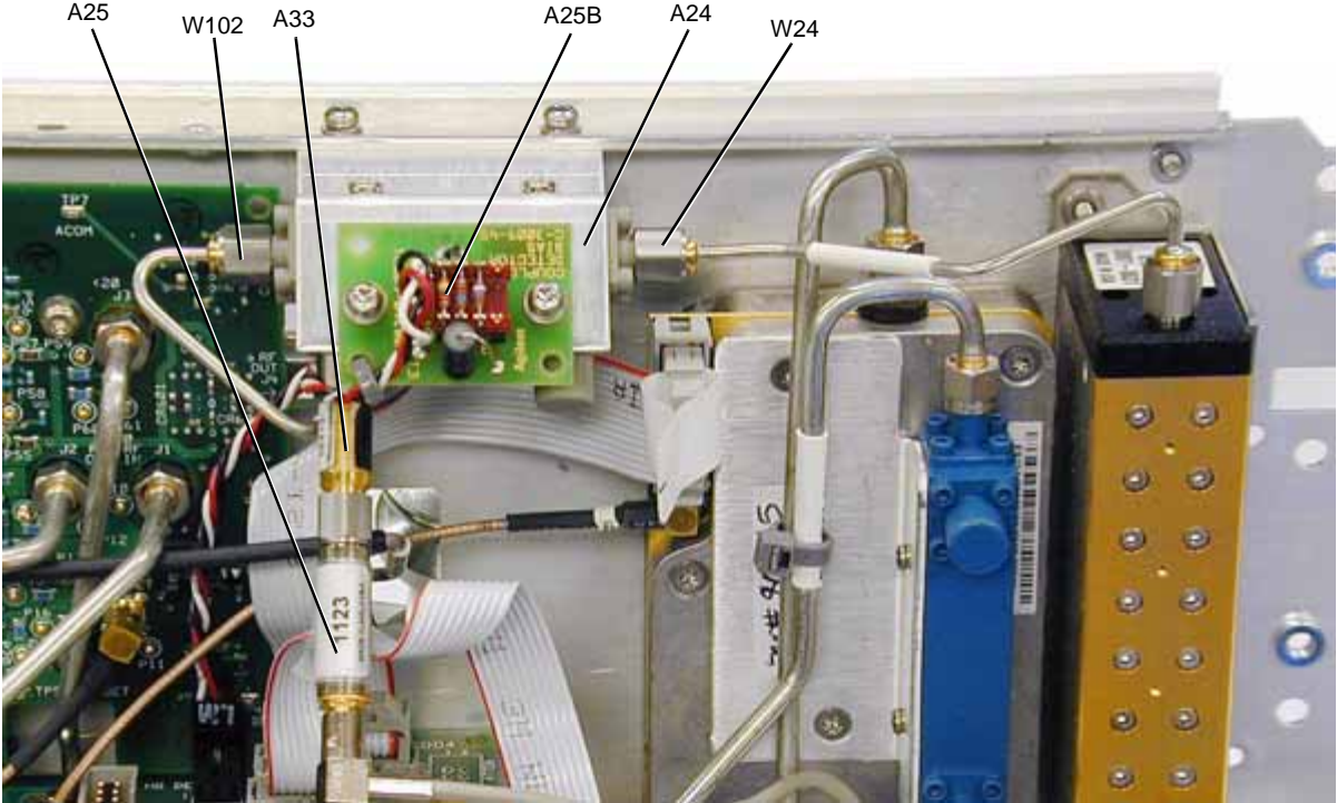
Figure 2-29 A24 50 GHz Highband Coupler (Option 532/544 and Option 1EM)
