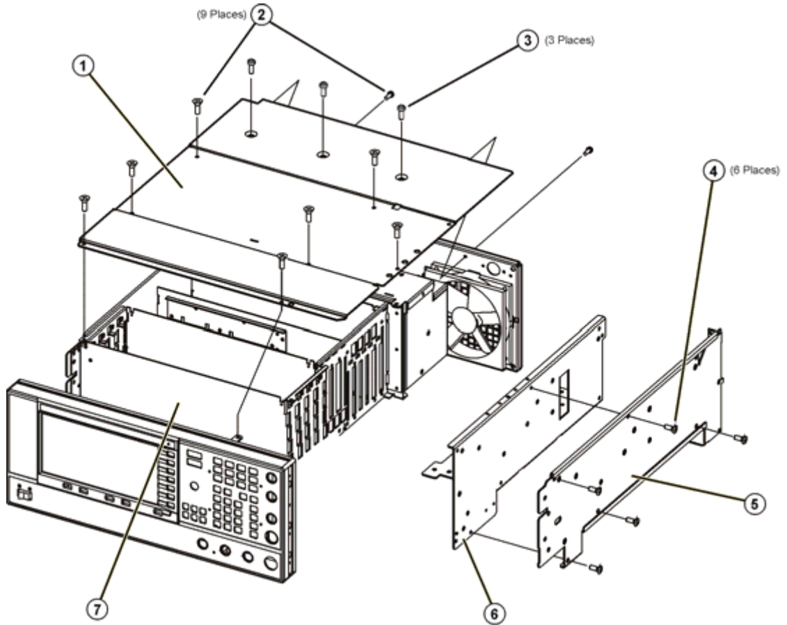
Figure 3-33 Main Chassis with Inside Cover and Right-Side Support Wall
